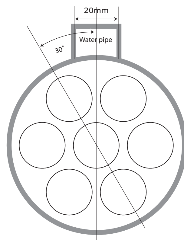
Water pipe position relative to air pipes
